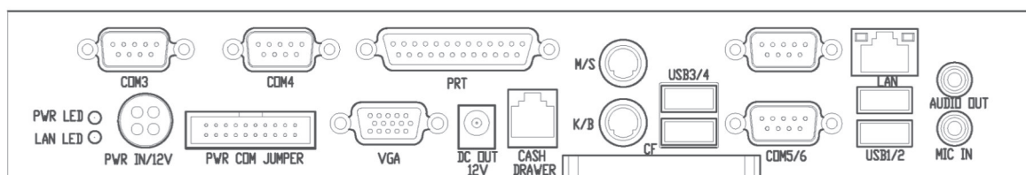
I/O Ports
